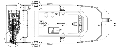
BRIDGE DECK DECK
